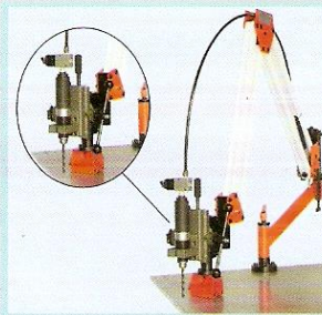
立式與水平氣動鑽孔座 Pneumatic Vertical and Horizontal Drilling / Tapping Device ADV-10 / ADVH-10
